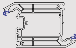
103366 115mm Open In Door Sash/Z Midrail
