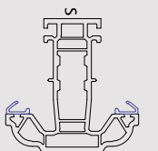
702533 70mm T Transom Et French Mullion
