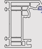
101164 60mm Outerframe
