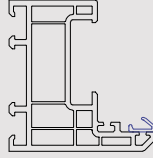
701591 68mm Outerframe
