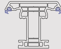
102268 86mm T Mullion
