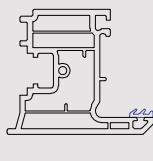
703592 68mm Reversible Sash
