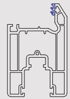
705151 90mm Patio Sash Bevelled
