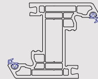
102269 86mm Z Mullion
