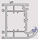
101161 70mm Outerframe
