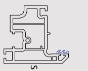
703810 61mm Flush Sash
