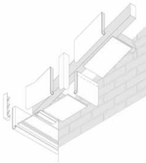
Box end detail (cut fascia board)
