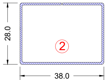
Outerframe
