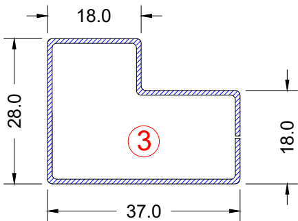
Lockstile Outer
