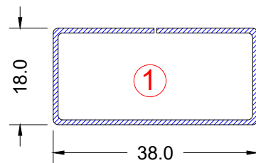
Outerframe
