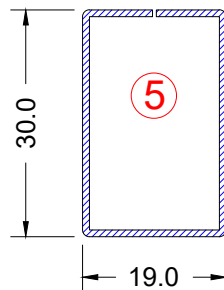
sash
