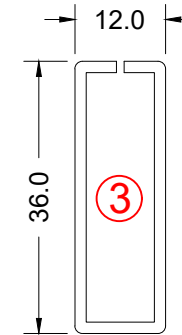
T &amp; Z mullion
