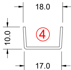
Outer frame
