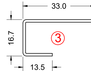
Ext Sash
