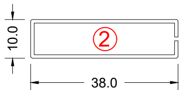
Outer/sash/transom
