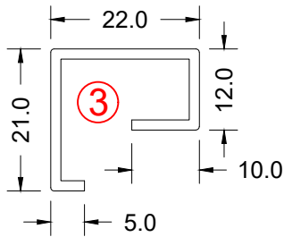
Casement Sash
