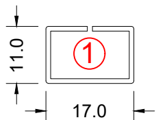
Small Outer
