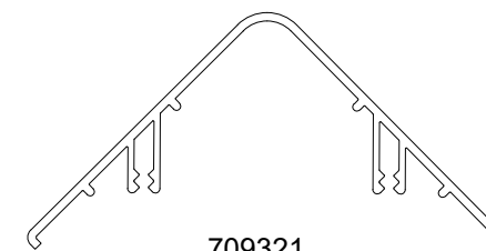
709321 90° Plain Post Cover
