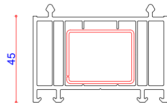
114062 45mm Frame Extension 35 x 28 Steel Box 713191
