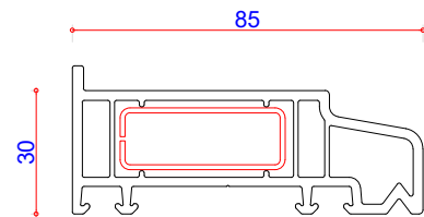
110122 85mm Cill 40 x 15 Steel Box 713016 End Caps 109258
