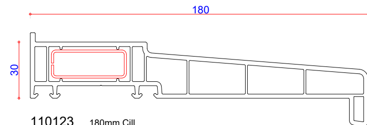
110123 180mm Cill 40 x 15 Steel Box 713016 End Caps 109259 Straight Coupler 109260
