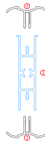
② APS16 - 16mm Coupler ⑦ APS-ST Small Trim
