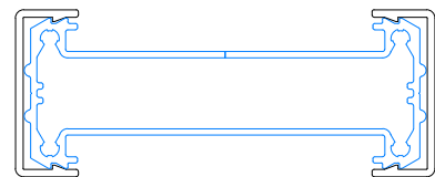
115117 20mm Vertical Aluminium Coupler 716323 Plain Cover
