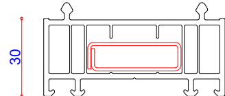
114061 30mm Frame Extension 36 x 11 Steel Box 113412 35 x 12 Steel Box 713187
