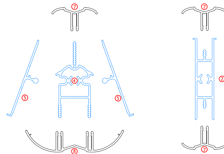
④ APS120 Variable Adaptor ⑤ APS120A Variable Bay Adaptor ⑧ APS-BT Bay Trim
